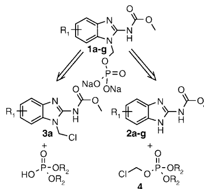
Scheme 1. Retrosynthetic approaches to 1
